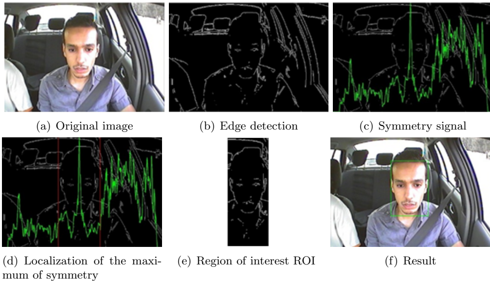
Fig. 3 Face detection using symmetry
