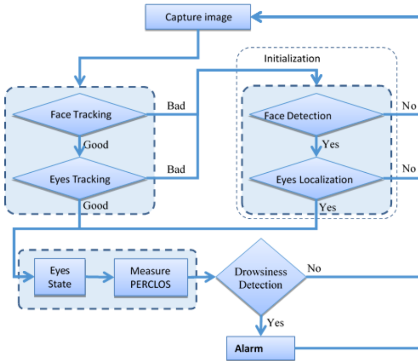
Fig. 1 Flowchart of the proposed system
