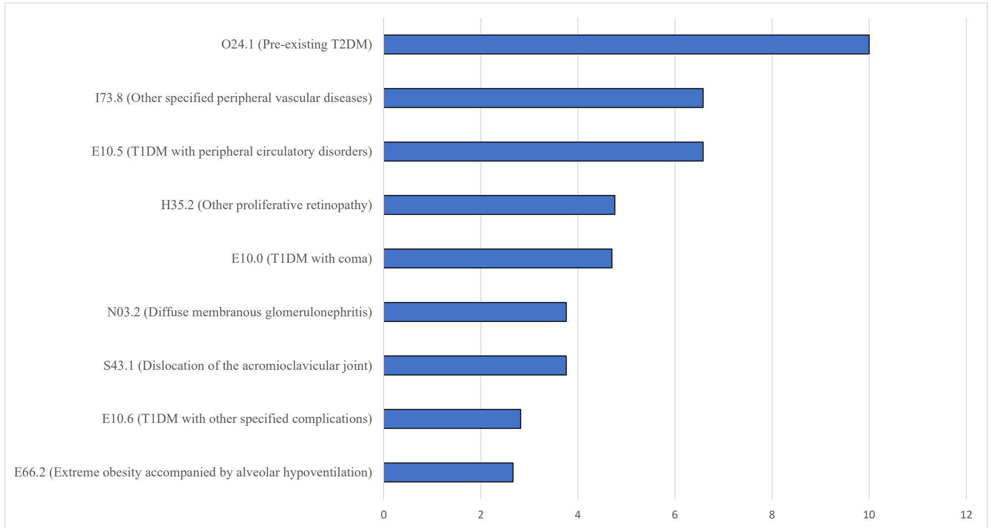
Fig. 4. Value of the conditional probability of non-random association ( conviction ) between existing diseases (9 diseases with the highest values) and T2DM (E11) in women.
