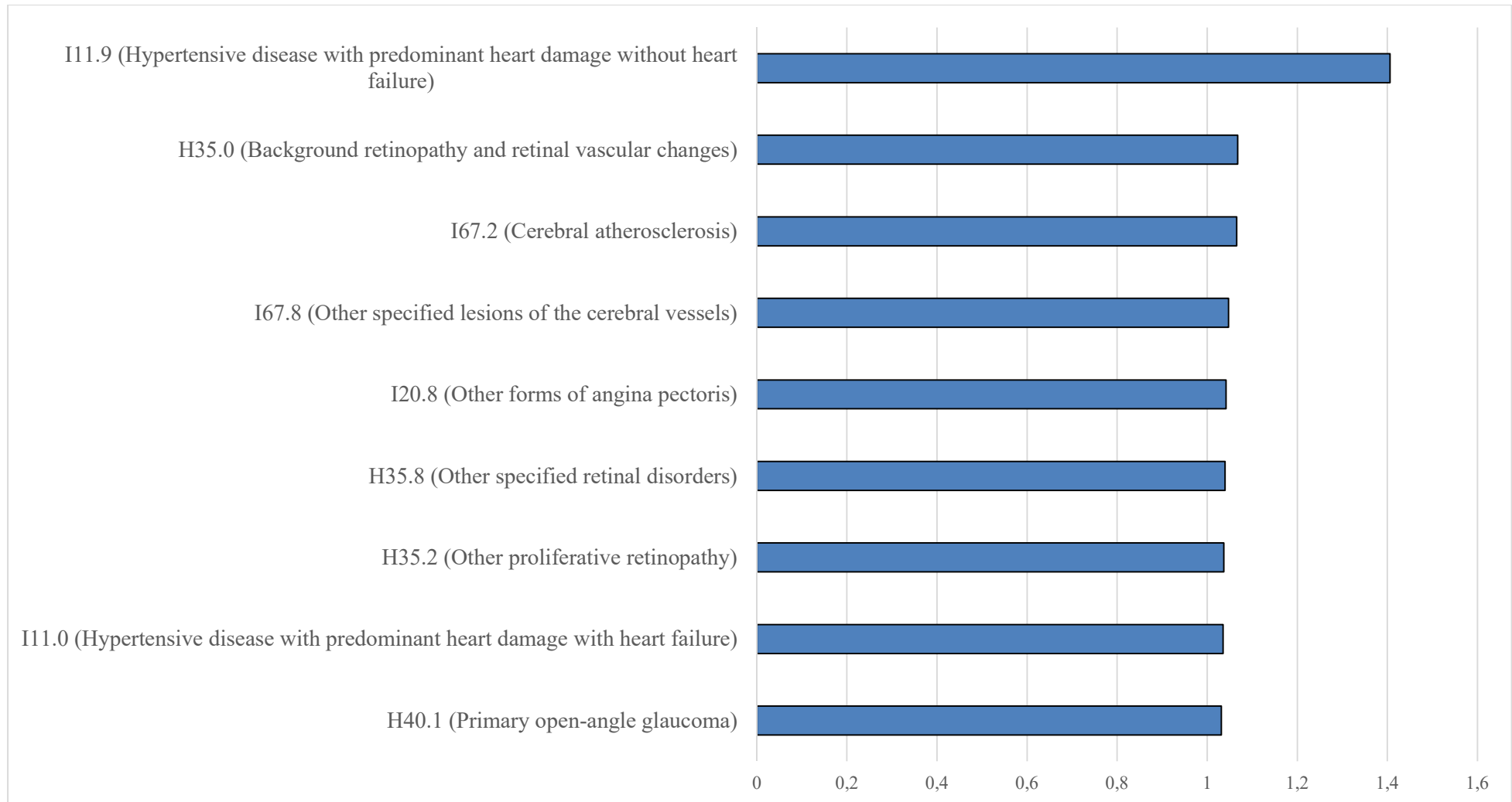
Fig. 2. Value of the conditional probability of non-random association ( conviction ) between existing T2DM (E11) and other diseases (9 diseases with the highest values) in women.
